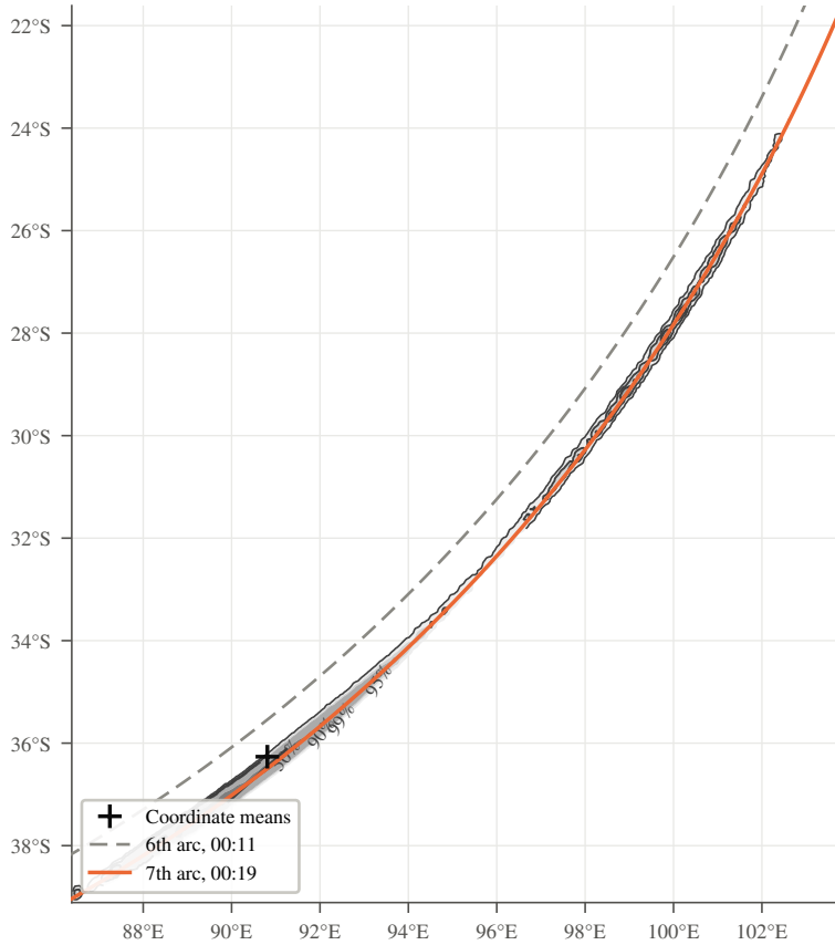
a Position at 00:19 UTC, over the 99% region
