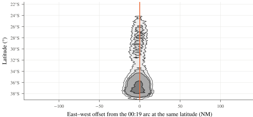
b The same posterior, measured from the arc
