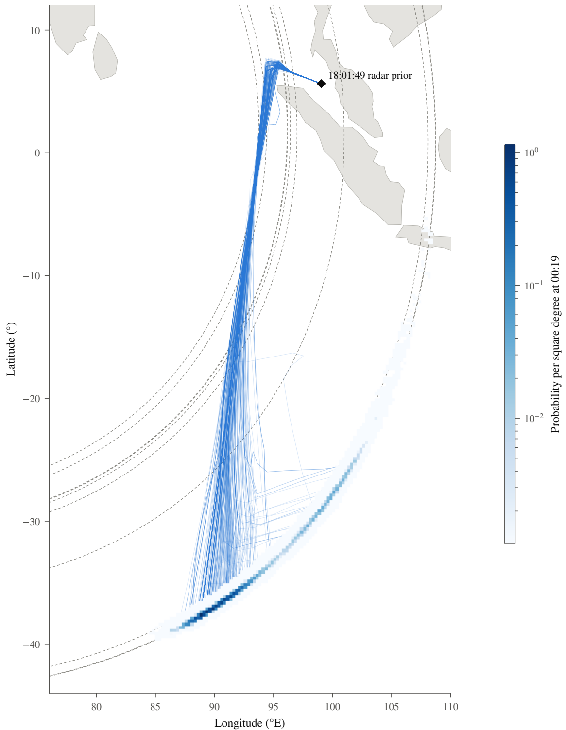
Figure 2. Posterior aircraft position at 00:19 UTC with BTO and BFO, pooled over 8 replicates (blue shading, logarithmic), and 400 routes drawn in proportion to posterior weight from replicate seed 1 (thin lines, 10-minute vertices). Dashed grey curves are the BTO arcs at a reference altitude of 35,000 ft; they are drawn for orientation only. Land: Natural Earth 1:110m.
